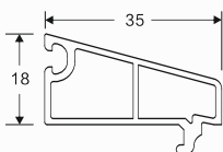
NAME: 60 single glazing bead A CODE: 60DYA WEIGHT(KG/M): 0.287 LENGTH: 5.8-6.0m PCS/BAG: 20 THICKNESS: 1.6 ②
