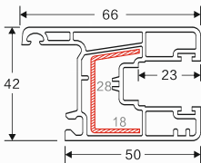
NAME: 88 sliding sash A2 CODE: 88TLSA2 WEIGHT(KG/M): 1.012 LENGTH: 5.8-6.0m PCS/BAG: 8 THICKNESS: 2.2
