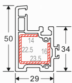
NAME: 60 casment / sliding mullion CODE: 60PKTLZT WEIGHT(KG/M): 0.665 LENGTH: 5.8-6.0m PCS/BAG: 6 THICKNESS: 2.3
