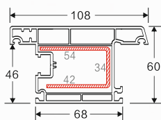
NAME: 60 out-swing door sash 2 CODE: 60WKMS2 WEIGHT(KG/M): 1.59 LENGTH: 5.8-6.0m PCS/BAG: 4 THICKNESS: 2.2 ②③
