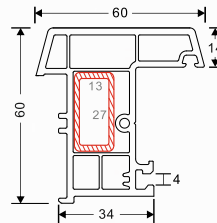
NAME: 60 lap joint CODE: 60DFZT WEIGHT(KG/M): 1.037 LENGTH: 5.8-6.0m PCS/BAG: 6 THICKNESS: 2.5 ②③
