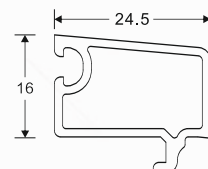
NAME: 88 glazing bead A CODE: 88DYA WEIGHT(KG/M): 0.24 LENGTH: 5.8-6.0m PCS/BAG: 20 THICKNESS: 2
