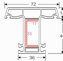
NAME: 60 mullion D CODE: 60ZTD WEIGHT(KG/M): 1.089 LENGTH: 5.8-6.0m PCS/BAG: 6 THICKNESS: 2.2 ②③④⑤⑥⑦⑧⑨
