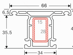
NAME: 42 sash mullion 2 CODE: 42SZT2 WEIGHT(KG/M): 0.78 LENGTH: 5.8-6.0m PCS/BAG: 8 THICKNESS: 2.2
