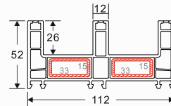
NAME: 60 double sliding frame A CODE: 60LGKA WEIGHT(KG/M): 1.098 LENGTH: 5.8-6.0m PCS/BAG: 6 THICKNESS: 2.2
