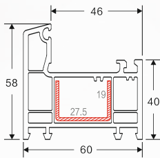
NAME: 60 frame D CODE: 60PKD WEIGHT(KG/M): 1.012 LENGTH: 5.8-6.0m PCS/BAG: 6 THICKNESS: 2.2 ②③④⑤⑥⑦⑧⑨
