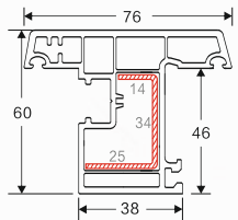
NAME: 60 out-swing window sash 2 CODE: 60WKCS2 WEIGHT(KG/M): 1.15 LENGTH: 5.8-6.0m PCS/BAG: 6 THICKNESS: 2.2 ②③④⑤⑥⑦⑧⑨
