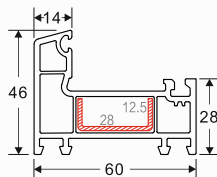
NAME: 60 small frame CODE: 60XK WEIGHT(KG/M): 0.85 LENGTH: 5.8-6.0m PCS/BAG: 6 THICKNESS: 2.2
