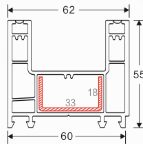
NAME: 60 double sliding frame A CODE: 60LGKA WEIGHT(KG/M): 1.098 LENGTH: 5.8-6.0m PCS/BAG: 6 THICKNESS: 2.2
