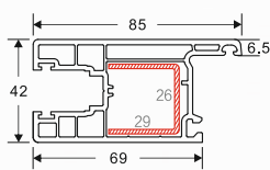
NAME: 60 sliding door sash 3 CODE: 60TLMS3 WEIGHT(KG/M): 1.22 LENGTH: 5.8-6.0m PCS/BAG: 4 THICKNESS: 2.2
