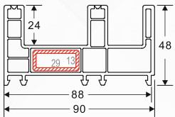
NAME: 90 sliding frame CODE: 90TLK WEIGHT(KG/M): 1.34 LENGTH: 5.8-6.0m PCS/BAG: 6 THICKNESS: 2.2
